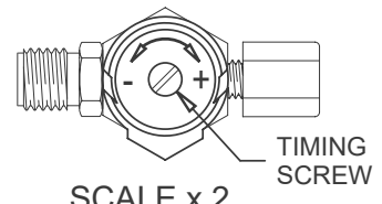
TOP VIEW ITEM #13
